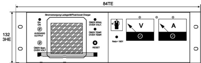
Depth: 380mm
