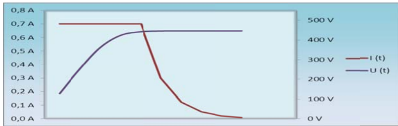
IU Characteristic
